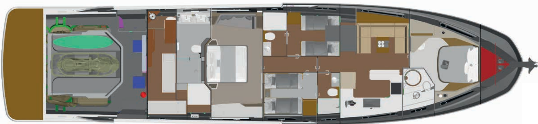
LOWER DECK
